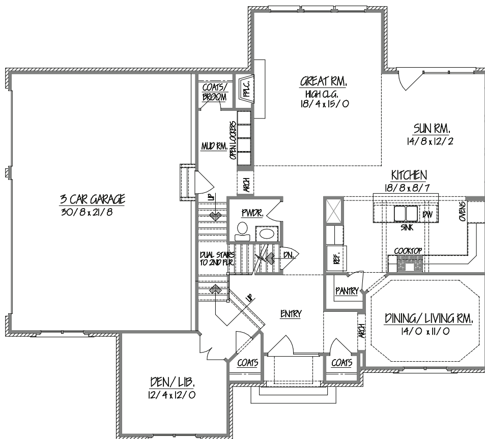
MAIN FLOOR 1,488 SQ. FT.
